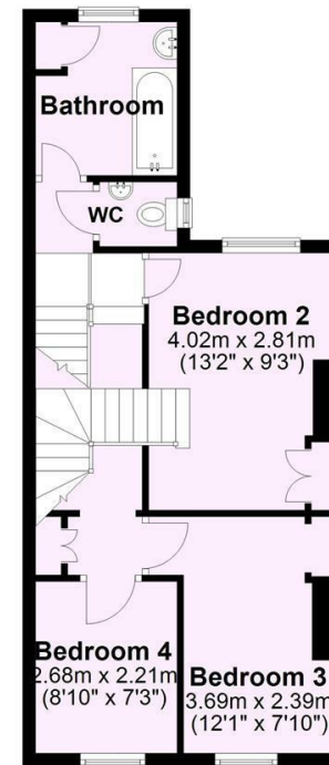
First Floor Approx. 44.2 sq. metres (475.3 sq. feet)
