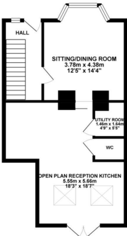
GROUND FLOOR 48.72 sq. m. ( 524.40 sq. ft. )
