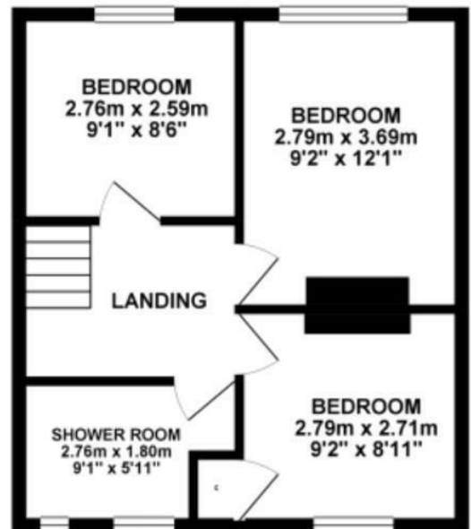
1ST FLOOR 35.53 sq. m. ( 382.47 sq. ft. )
