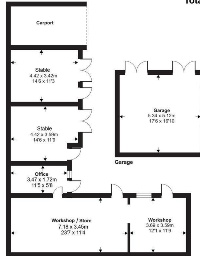
Stables/Workshop
