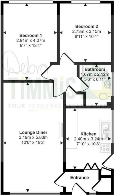
Floorplan
