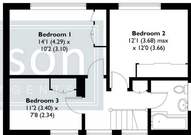
FIRST FLOOR 497 SQ FT / 46.2 SQ M
