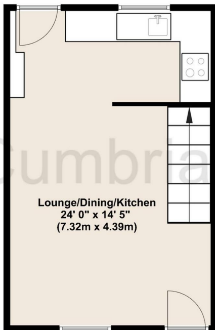
Ground Floor Approx 31.00 Sq meters (334.00 Sq feet).
