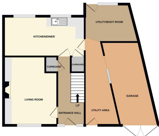
GROUND FLOOR 768 sq.ft. (71.3 sq.m.) approx.
