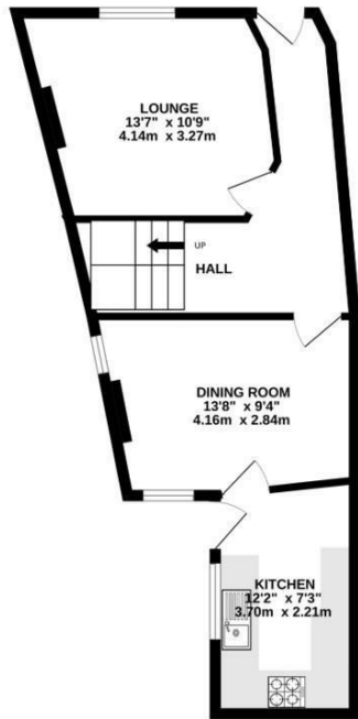
GROUND FLOOR 432 sq.ft. (40.1 sq.m.) approx.
