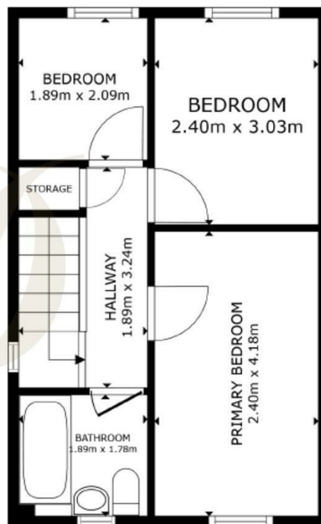
FLOOR 2
