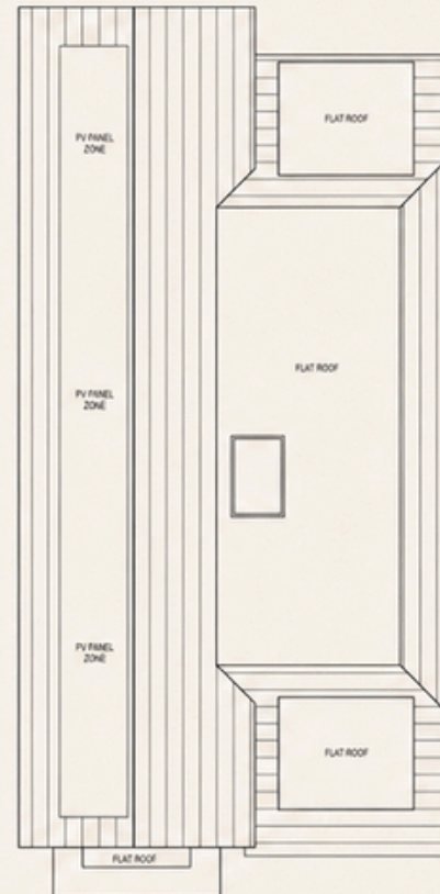
ROOF PLAN
