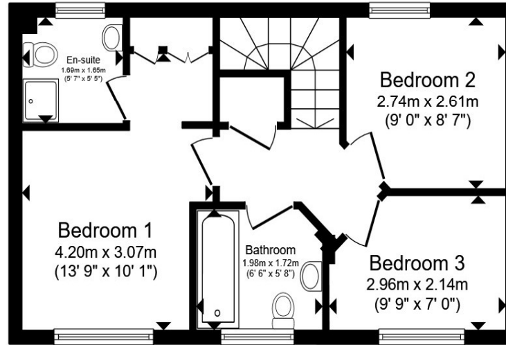
First Floor
