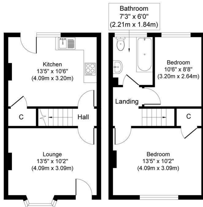
Ground Floor Approximate Floor Area 326 sq. ft (30.26 sq. m)
