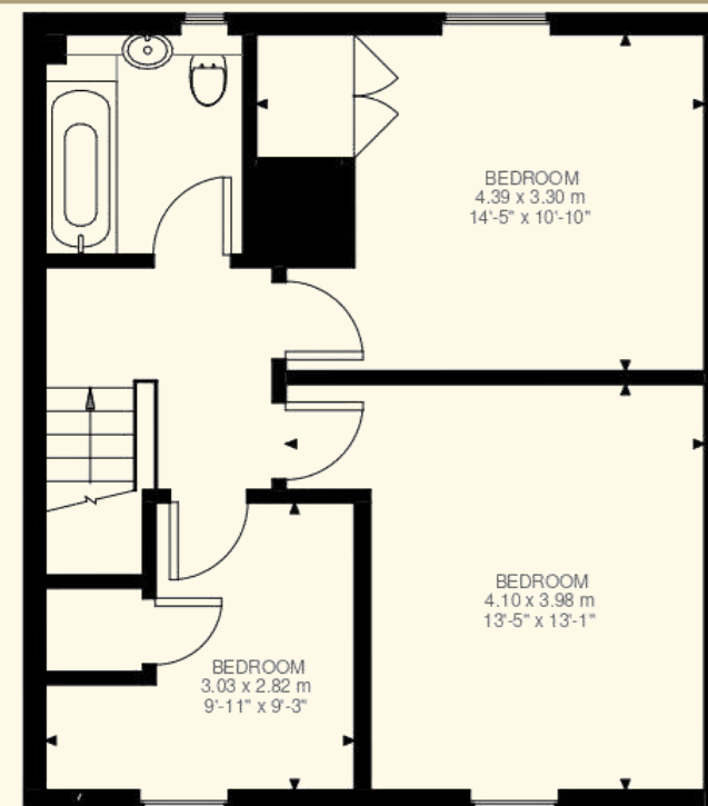
First Floor 517 ft²
