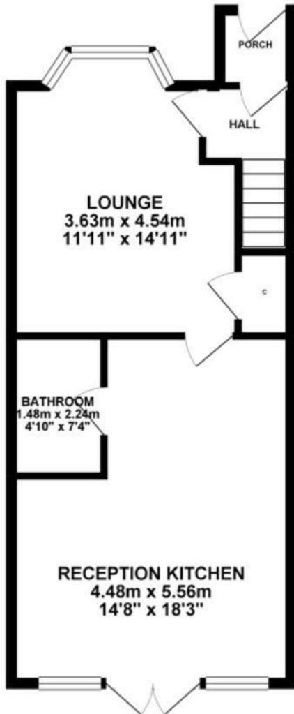
GROUND FLOOR 45.06 sq. m. ( 485.01 sq. ft. )
