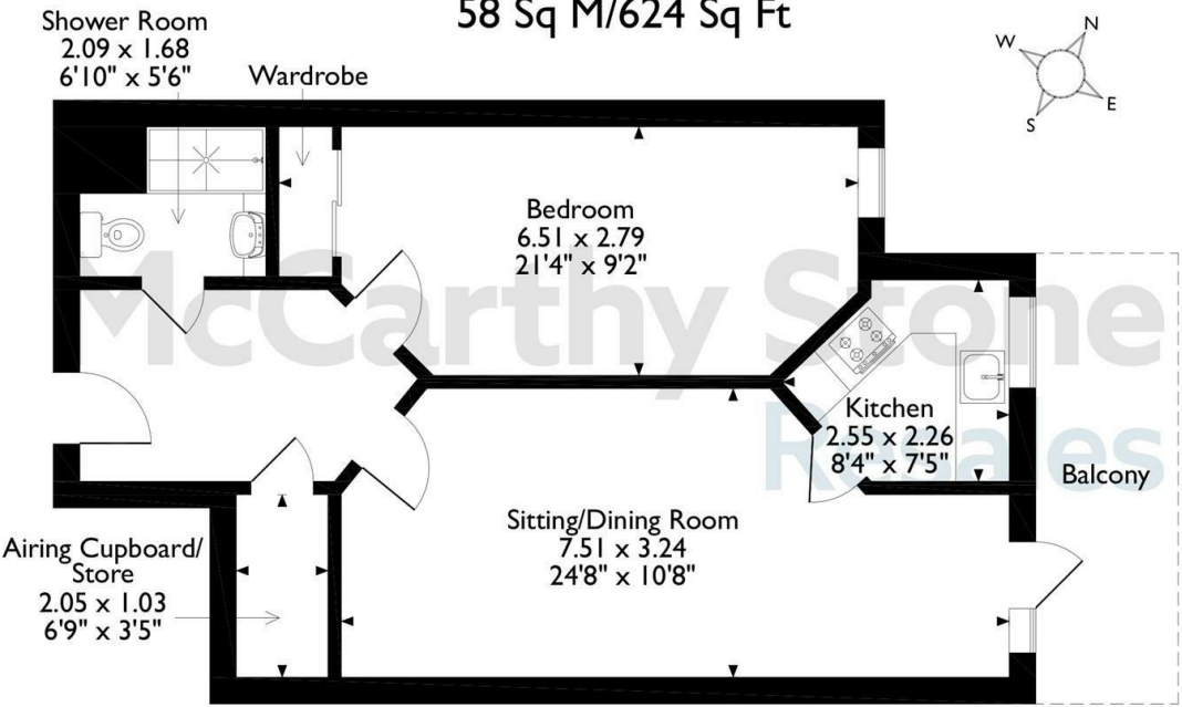
Level 2 Flat
