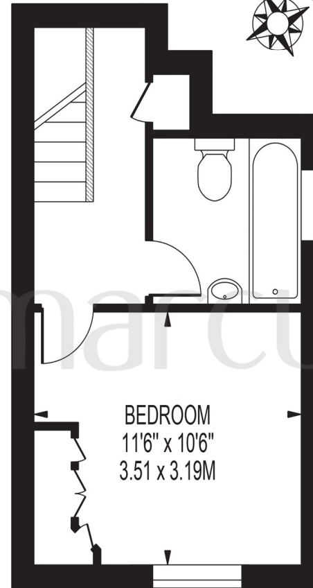
THIRD FLOOR
