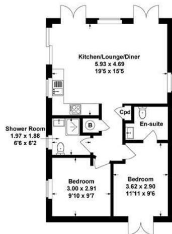
Chalet 58.0 sq m / 624 sq ft
