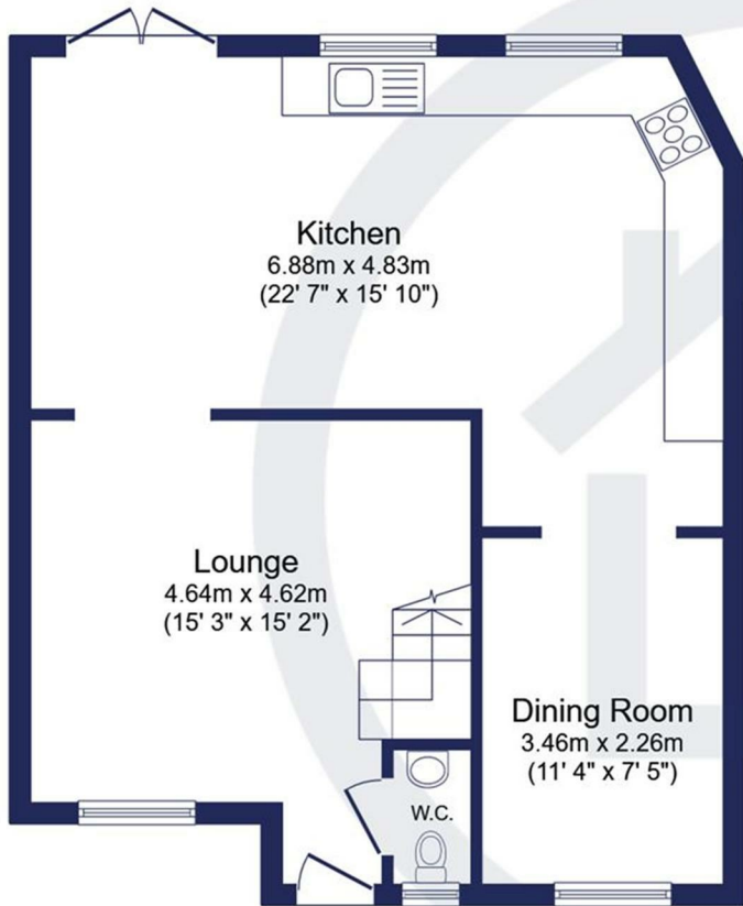
Ground Floor Floor area 56.5 sq.m. (608 sq.ft.)
