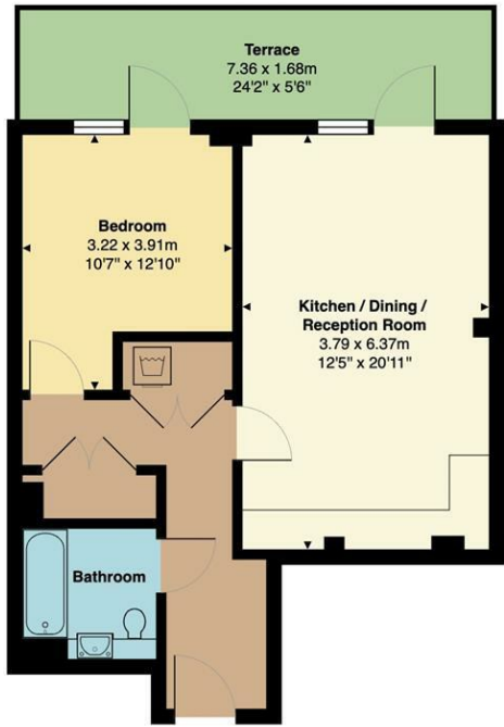
Total Area: 53.1 m 2 ... 572 ft 2 (excluding terrace) All measurements are approximate and for display purposes only
