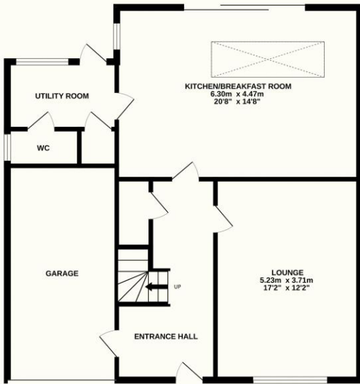
GROUND FLOOR 85.6 sq.m. (922 sq.ft.) approx.
