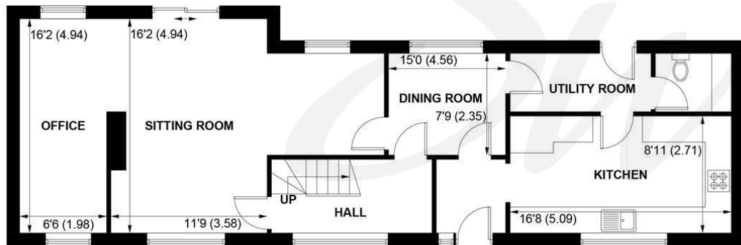
GROUND FLOOR
