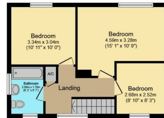
First Floor Floor area 45.4 sq.m. (489 sq.ft.)
