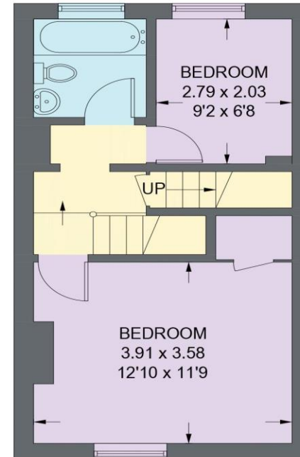
FIRST FLOOR 32.0 SQ M / 344 SQ FT
