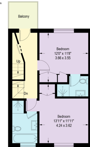
Fourth Floor
