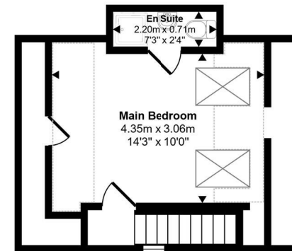
Second Floor Approx 25 sq m / 269 sq ft
