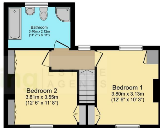
First Floor Floor area 36.3 sq.m. (390 sq.ft.)
