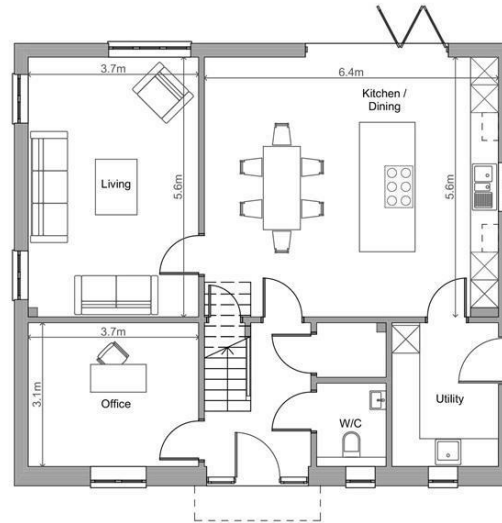
Ground Floor 1:100
