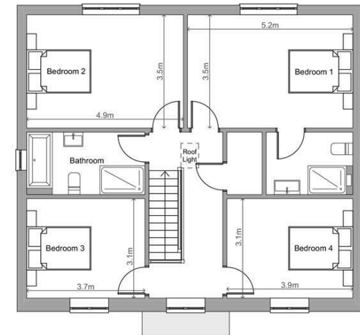
First Floor 1:100
