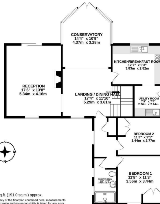
FIRST FLOOR 1110 sq.ft. (103.1 sq.m.) approx.
