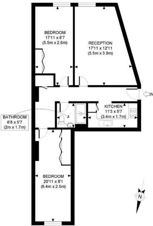
SECOND FLOOR GROSS INTERNAL FLOOR AREA 767 SQ FT APPROX. GROSS INTERNAL FLOOR AREA: 767 SQ FT/ 71 SQM
