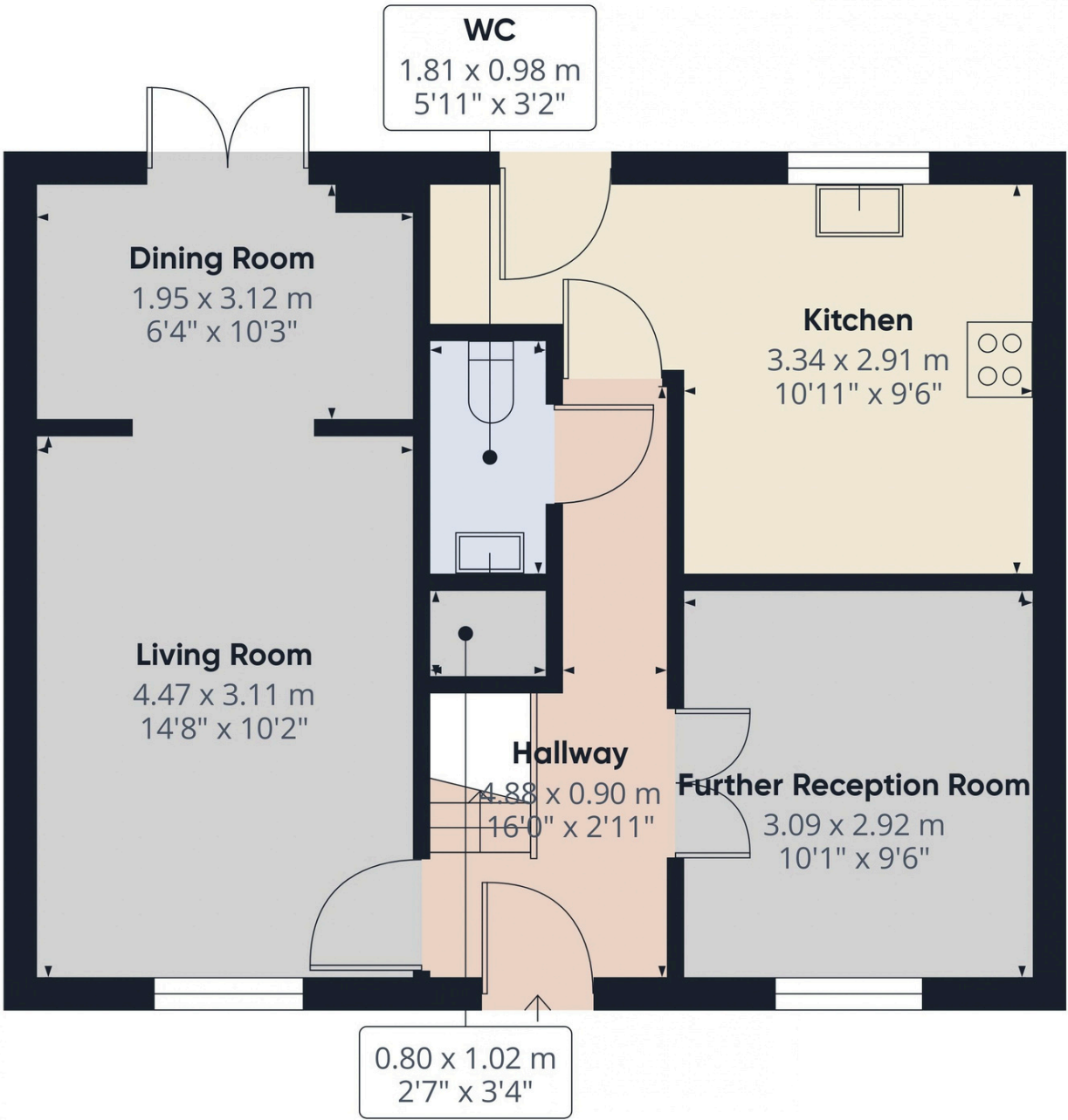
Ground Floor
