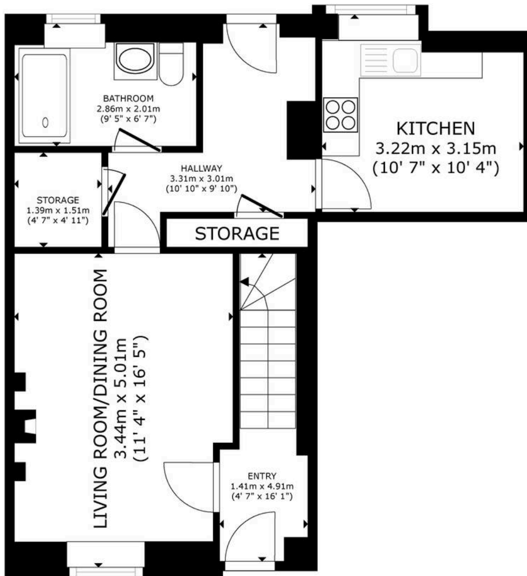
FLOOR 1
