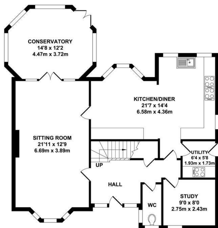
GROUND FLOOR APPROX. FLOOR AREA 1019 SQ.FT. (94.68 SQ.M.)
