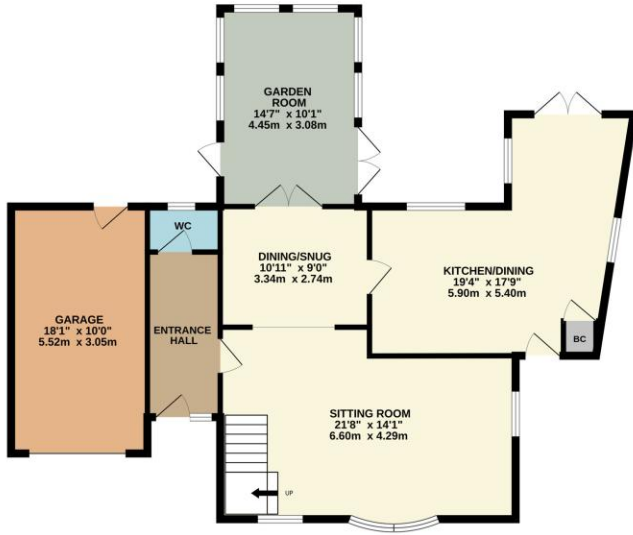
GROUND FLOOR 1043 sq.ft. (96.9 sq.m.) approx.
