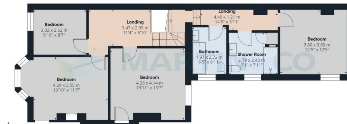
Floor 1
