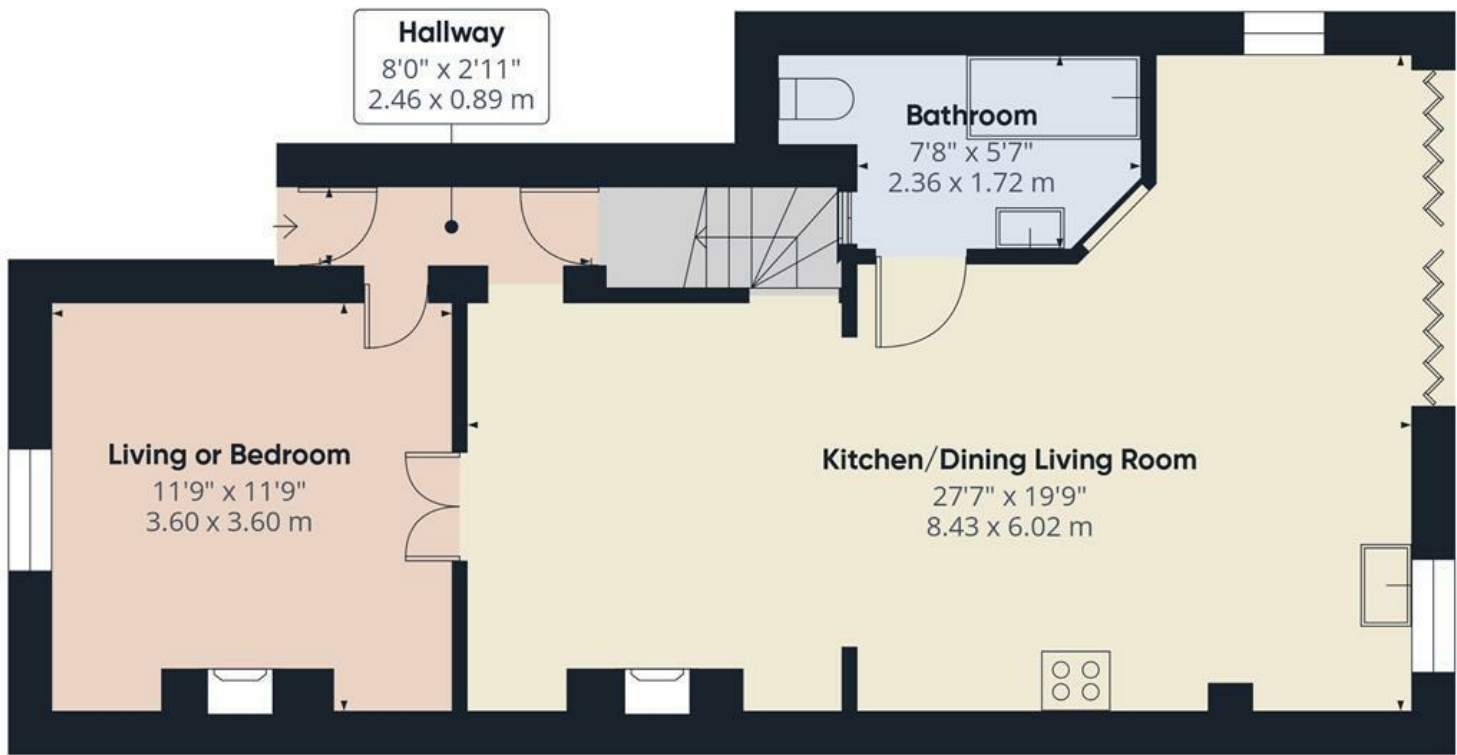
Ground Floor
