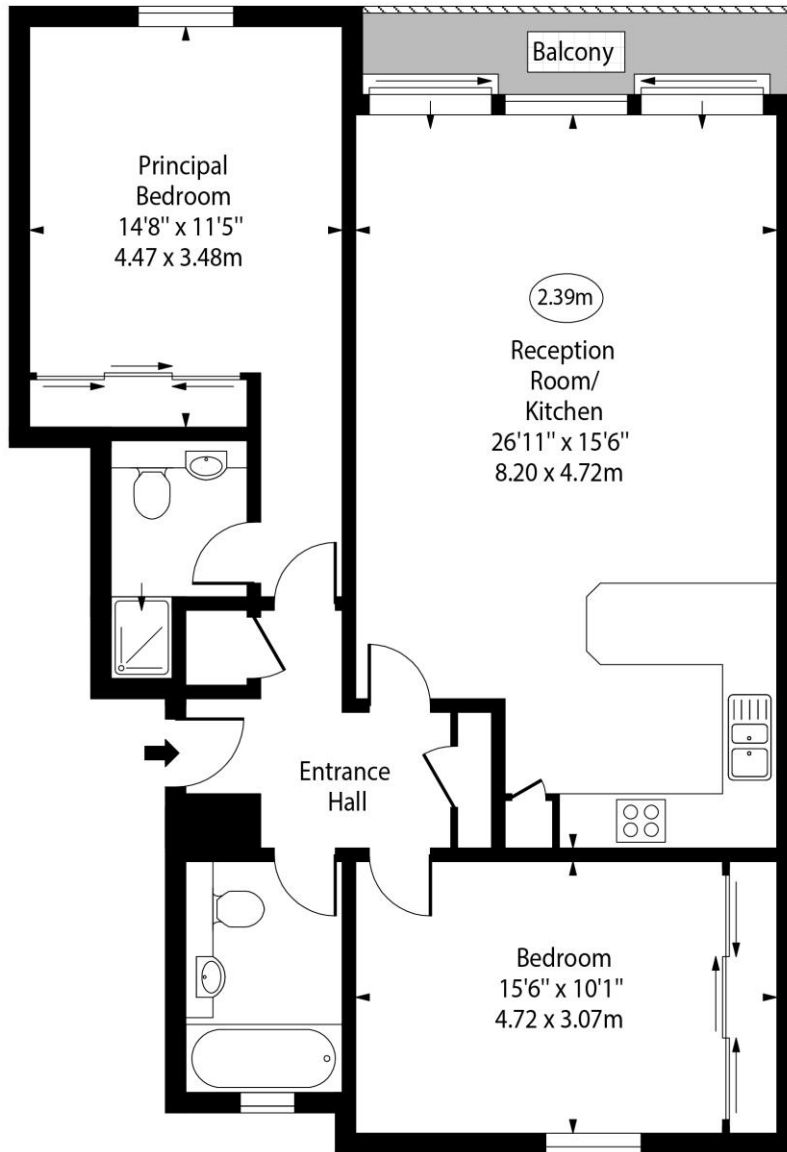
Second Floor
