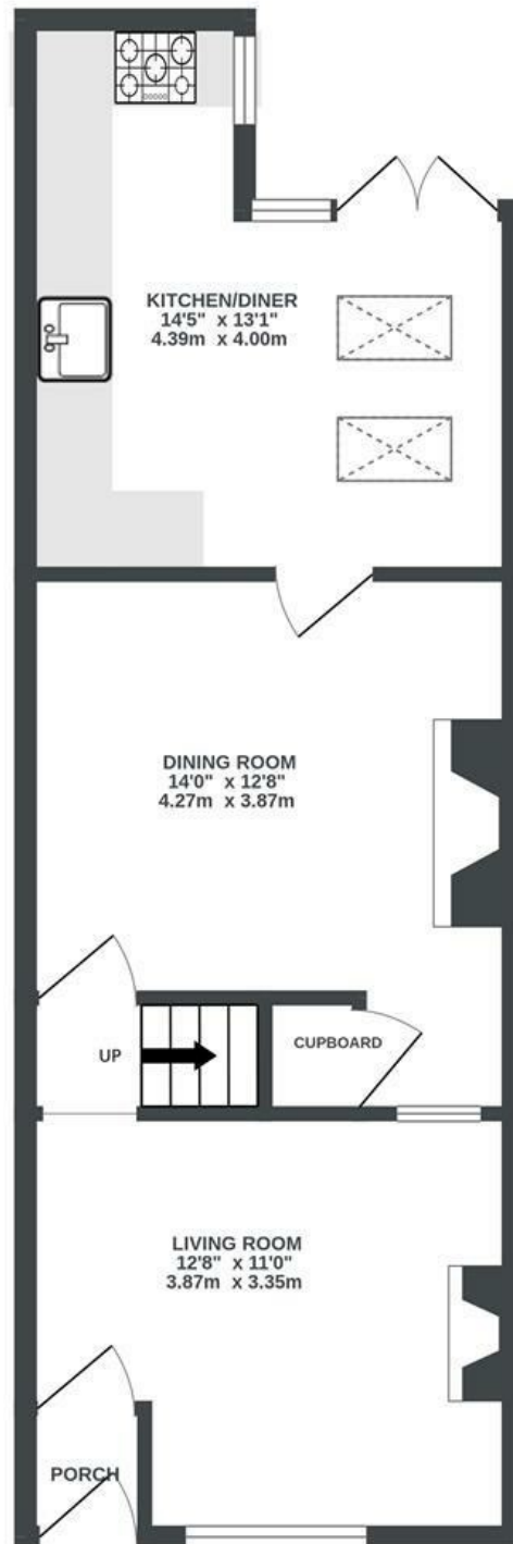
GROUND FLOOR
