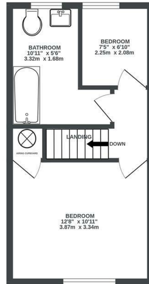
1ST FLOOR
