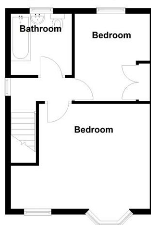
First Floor Approx. 34.9 sq. metres (375.6 sq. feet)
