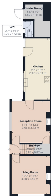
Floor 0 Building 1
