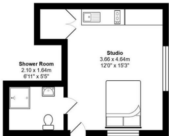
Belmont Road, Wallington, SM6 8TE (Ground Floor 11)
