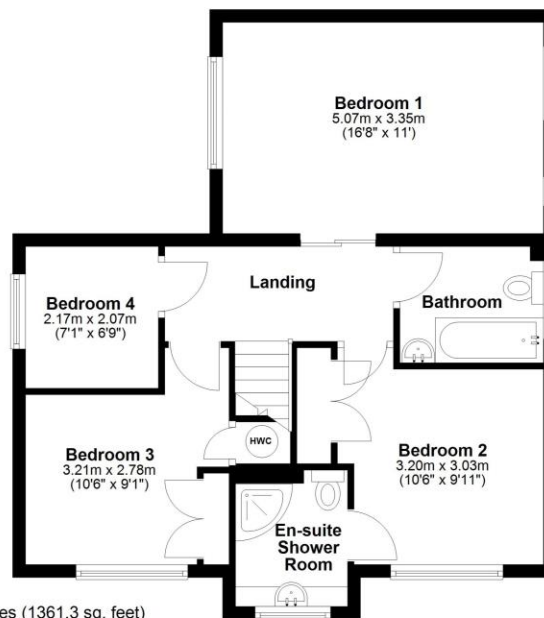
First Floor Approx. 57.8 sq. metres (622.1 sq. feet)
