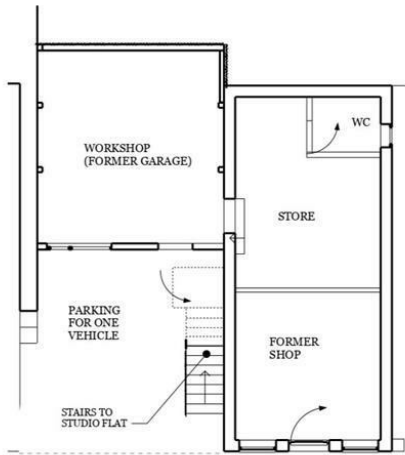
6 EXISTING GROUND FLOOR PLAN B4 2100
