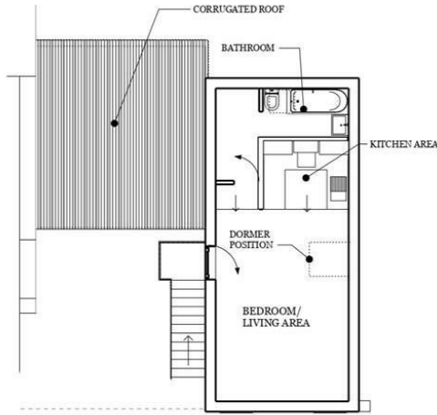
7 EXISTING FIRST FLOOR PLAN B4 2100
