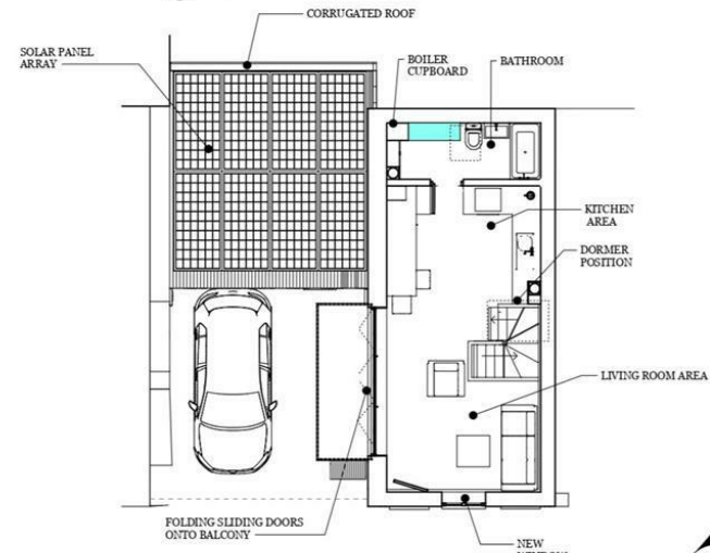
9 PROPOSED FIRST FLOOR PLAN B4 2100
