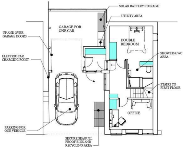
8 PROPOSED GROUND FLOOR PLAN B4 2100
