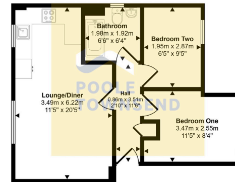
Floorplan
