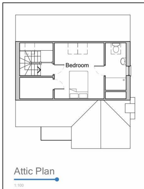
ATTIC PLAN
