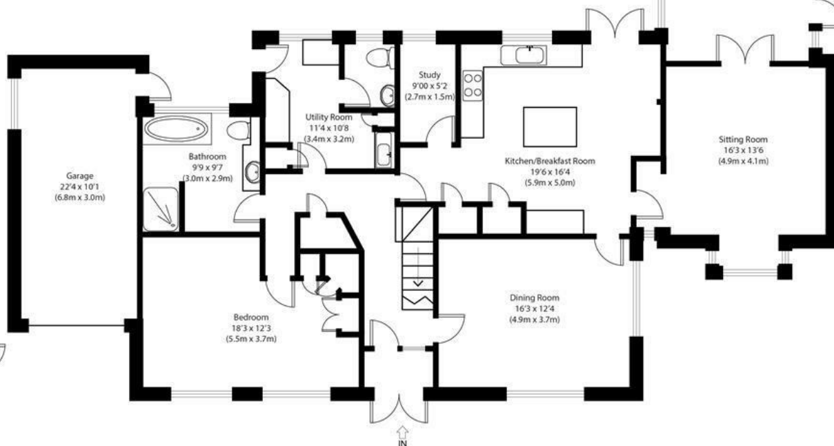
Ground Floor
