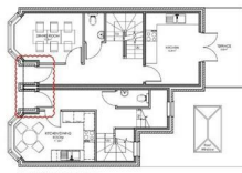
GROUND FLOOR PLAN - PLOT 1
