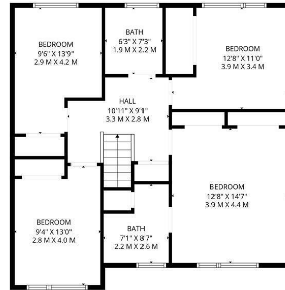
2ND FLOOR
