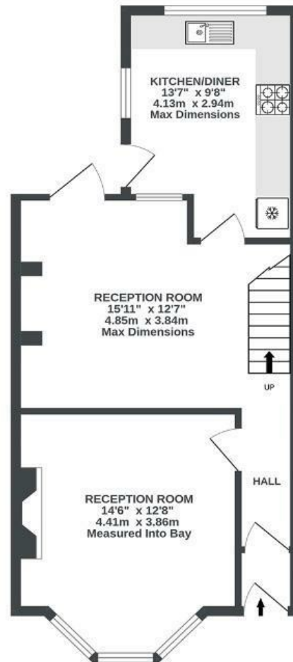
GROUND FLOOR 501 sq.ft. (46.6 sq.m.) approx.
