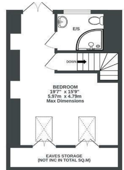
2ND FLOOR 276 sq.ft. (25.6 sq.m.) approx.
