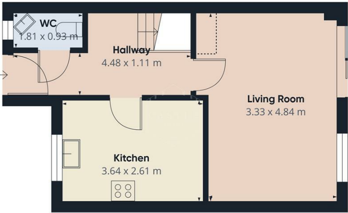
Floor 0
