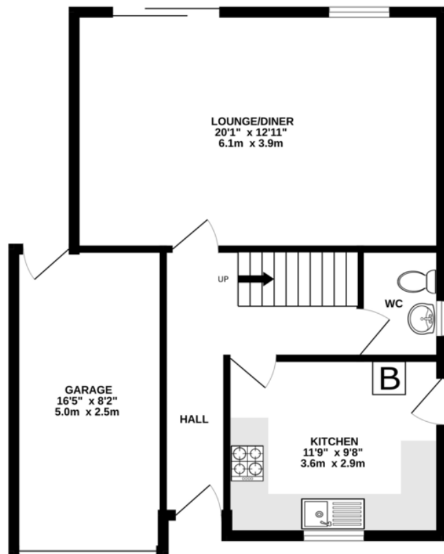
GROUND FLOOR 625 sq.ft. (58.0 sq.m.) approx.
